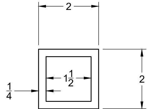
SCALE 1:2 Side
